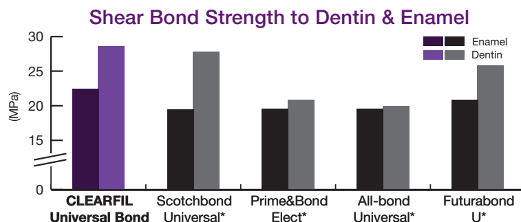
Fig. 1 Shear Bond Strength on Dentin and Enamel in self-etch mode
